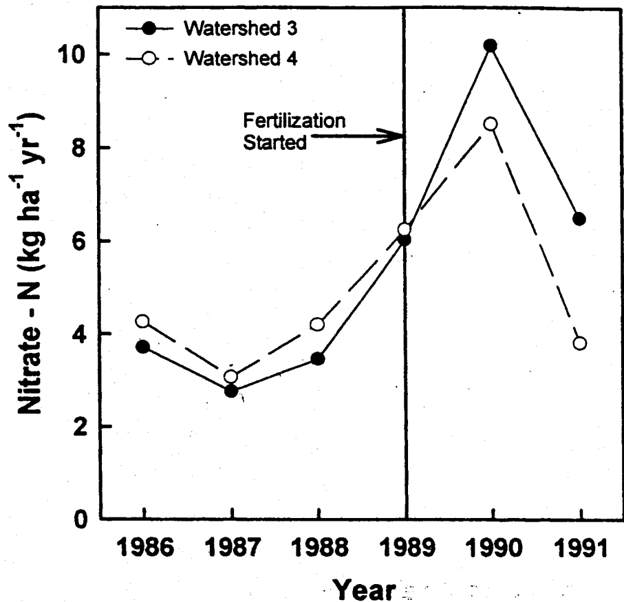
Figure 6. Annual discharge of nitrate in stream water leaving Watersheds 3 and 4 at the Fernow Experimental Forest (from Adams et al. 1993). The value for Watershed 3 in 1991 is corrected for an error in the original article (M.B. Adams, pers. comm.). Watersheds 3 and 4 were last cut in 1972 and 1905 respectively. Aerial fertilization with 35 \text{ kg N ha}^{-1} \text{ yr}^{-1} in 3 applications of ammonium sulfate was begun on Watershed 3 in 1989. Watershed 4 has not been fertilized.
