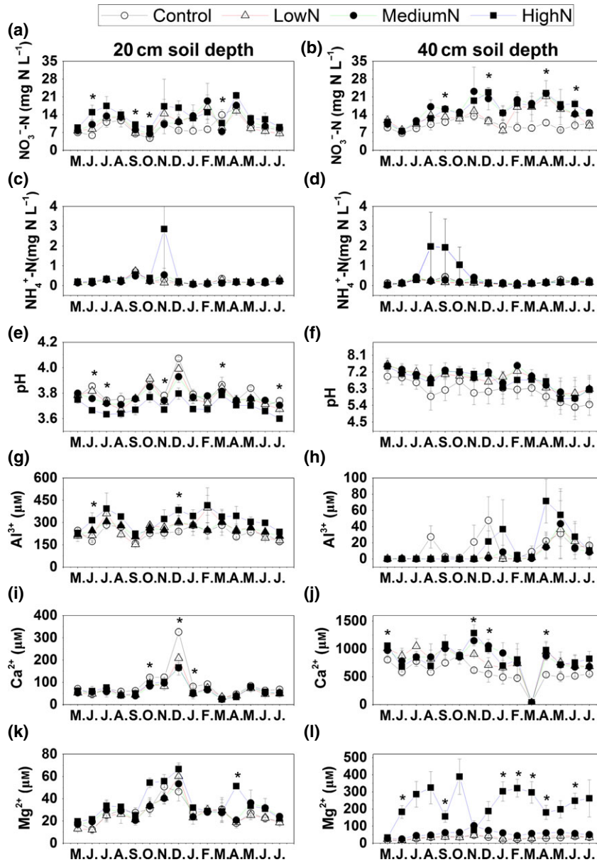
Fig. 7 Responses of \text{NO}_3^- -N (a, b), \text{NH}_4^+ -N (c, d), pH (e, f), \text{Al}^{3+} (g, h), \text{Ca}^{2+} (i, j) and \text{Mg}^{2+} (k, l) dynamics to long-term N addition in soil solutions at 20 cm (left panel) and 40 cm (right panel) soil depth. Water samples were taken from May 2009 to July 2010. Asterisks (*) indicates that there are significant differences at P < 0.05 levels between N treatments and the Controls using planned contrast analysis.
