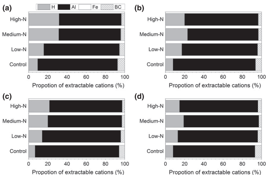
Fig. 4 Effects of long-term N additions on relative composition of soil exchangeable cations (percentage charge of total CEC) in 0–10 cm (a), 10–20 cm (b), 20–30 cm (c) and 30–40 cm (d) soils. Note: BC, the total base cations of \text{K}^+ , \text{Na}^+ , \text{Ca}^{2+} and \text{Mg}^{2+} .
