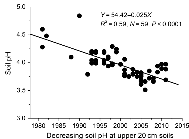
Fig. 1 Soil pH_{(water)} changing trend at upper 20 cm soils during the last three decades in the lowland tropical forest (monsoon evergreen broadleaf forest) of Dinghushan Biosphere Reserve in Southern China. Note: The data set used here was compiled from the published papers, which focused on the same forest to this study. The upper 20 cm of the mineral soil (below the forest floor) was sampled. Method for determination of soil pH is the same as this study, using the national standard of China (GB7859-87). These published papers are listed in Data S2.
