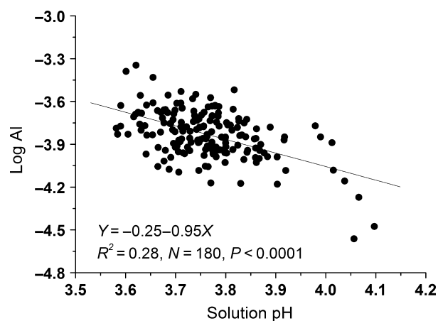
Fig. 8 Relationships between the activities of Al and pH in the solutions at 20 cm soil depth across all plots during the study period.
