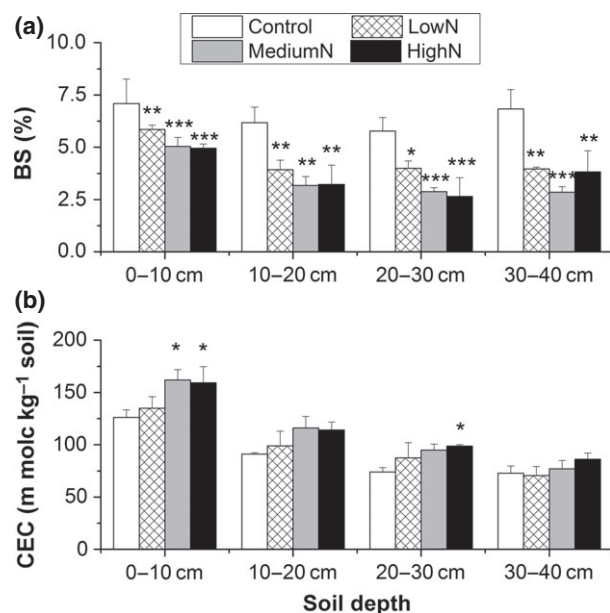
Fig. 5 Responses of soil base saturation (BS, (a) and cation exchange capacity (CEC, (b) to elevated N addition in the lowland tropical forest of Southern China. Asterisks (*), (** and (***) indicate that there are significant differences at P < 0.1 , P < 0.05 and P < 0.01 levels between N treatments and the Controls, respectively.
