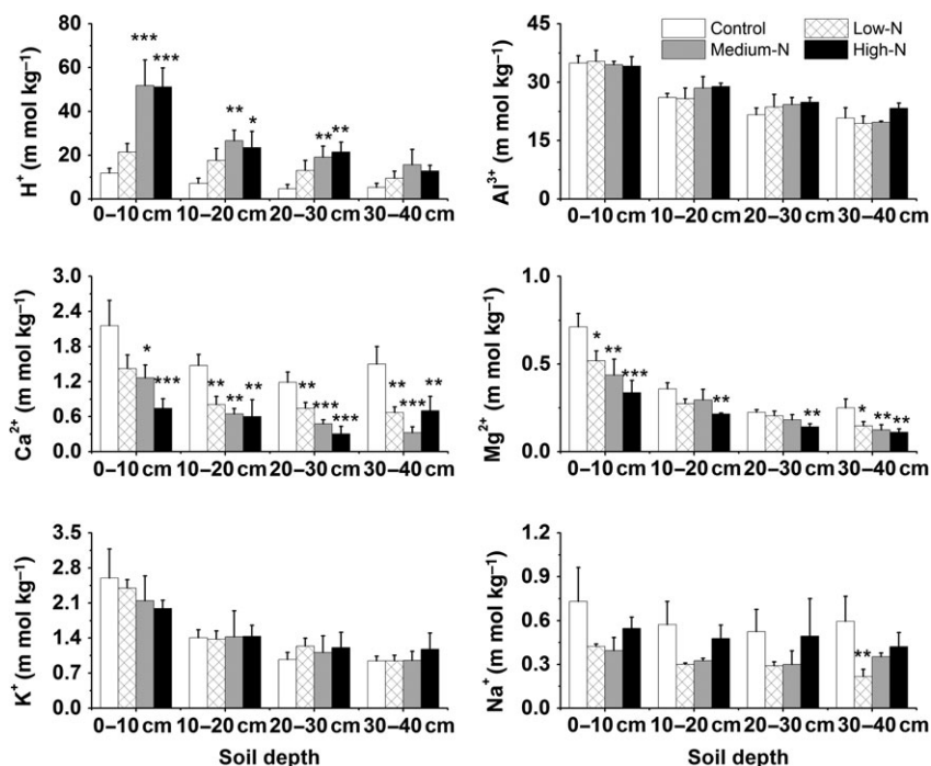
Fig. 3 Responses of soil exchangeable cations to long-term N addition in the lowland tropical forest of Southern China. Asterisks (*), (**) and (***) indicate that there are significant differences at P < 0.1 , P < 0.05 and P < 0.01 levels between N treatments and the Controls, respectively.
