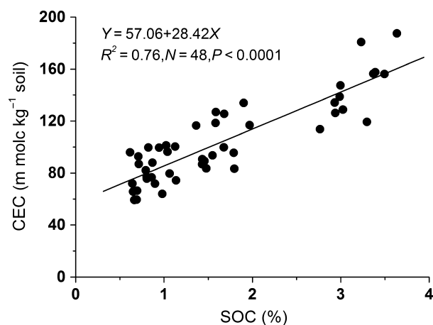
Fig. 6 Relationships between soil cation exchange capacity (CEC) and soil organic carbon (SOC) across all plots along the whole soil profiles from 0–40 cm depth.
