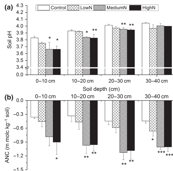
Fig. 2 Responses of soil pH and water-extracted acid neutralizing capacity (ANC) to long-term N addition in the lowland tropical forest of Southern China. Note : Error bar means standard error; Asterisks (*), (**) and (***) indicate that there are significant differences at P < 0.1 , P < 0.05 and P < 0.01 levels between N treatments and the Controls, respectively.
